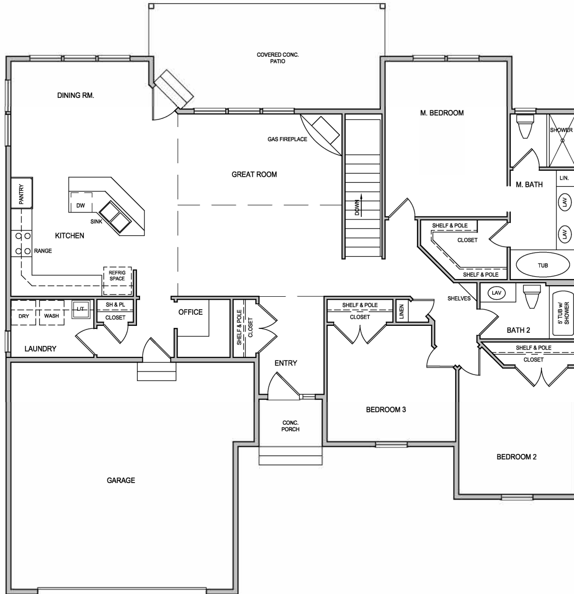
FLOOR PLAN
