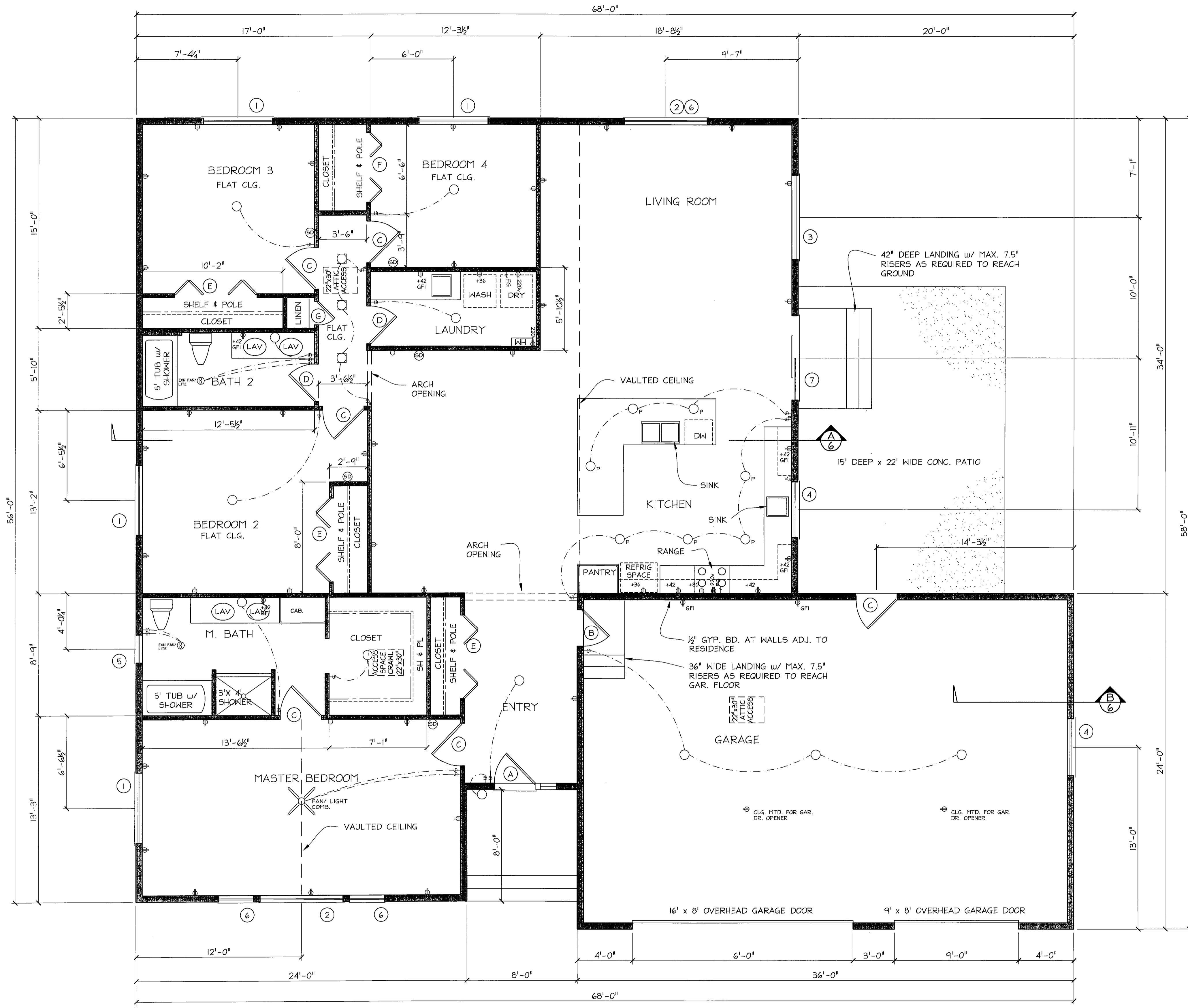
MAIN FLOOR PLAN SCALE: 1/4" = 1'-0"
